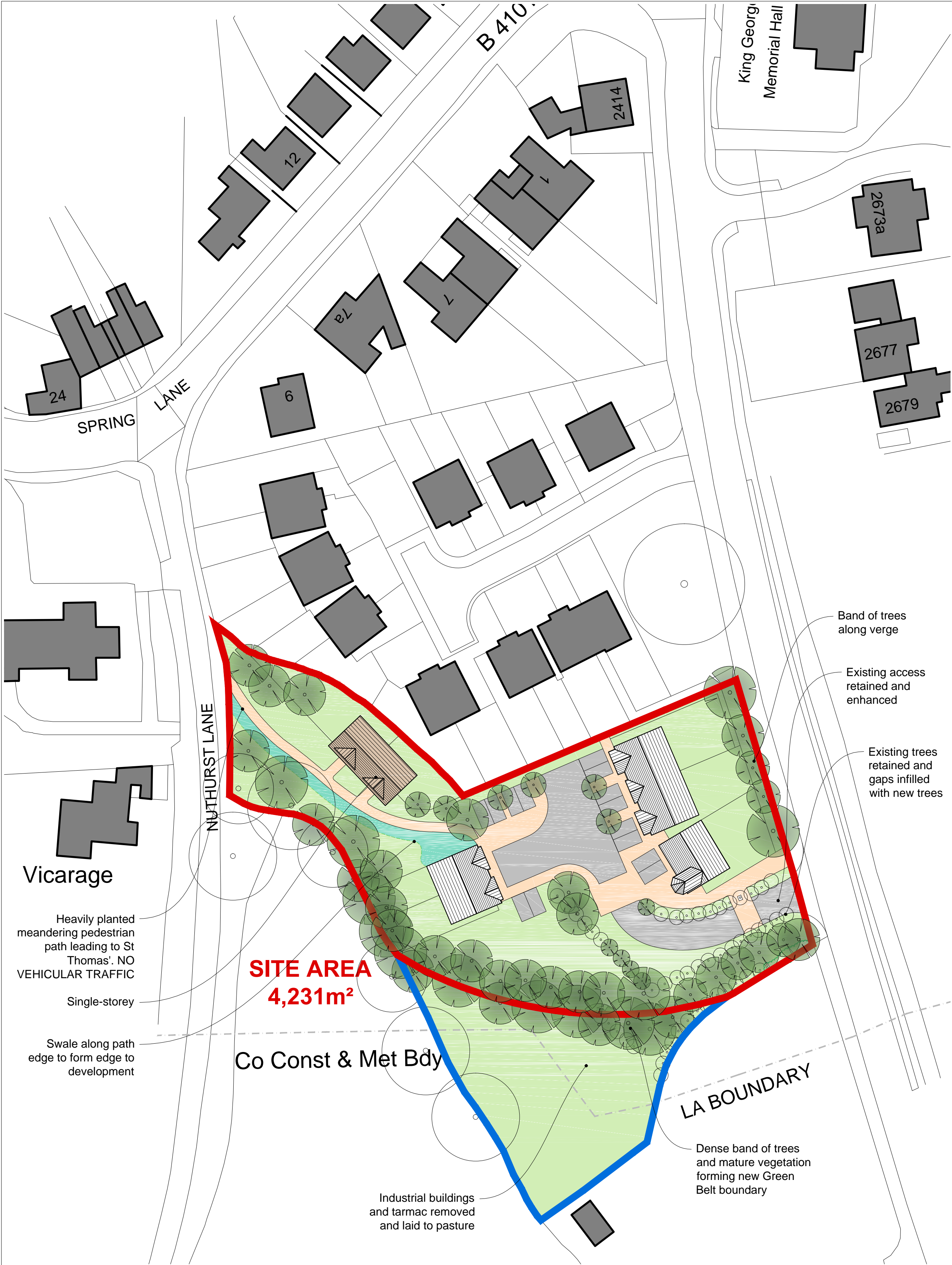
02 Proposed Layout Plan Scale 1:500@A1
